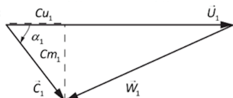
Figure 2: velocity triangle at the inlet
