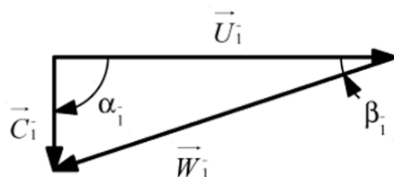
Figure 3: velocity triangle at the outlet
